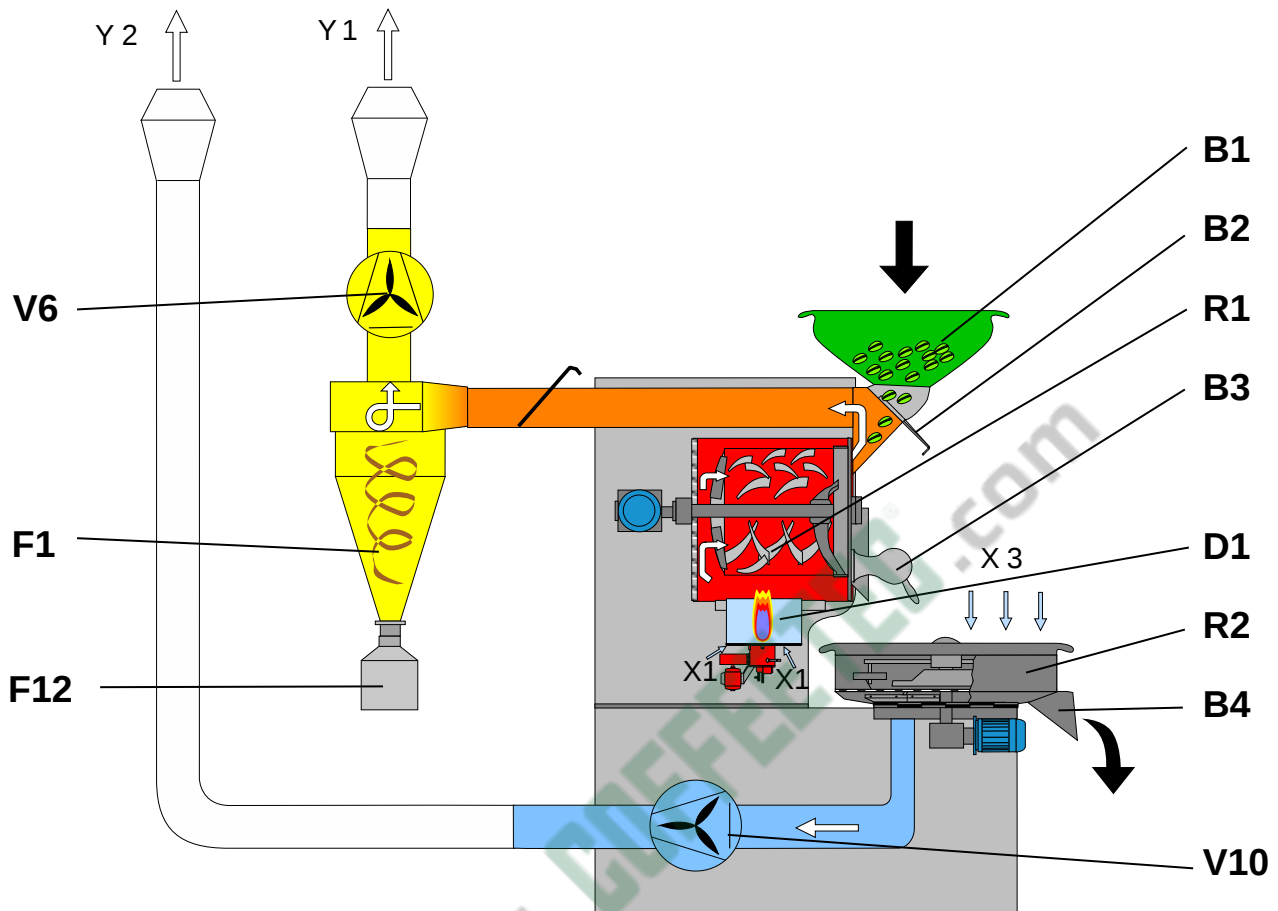
Illustration 2: Process scheme (variant 2: roasting/cooling exhaust air separated)
