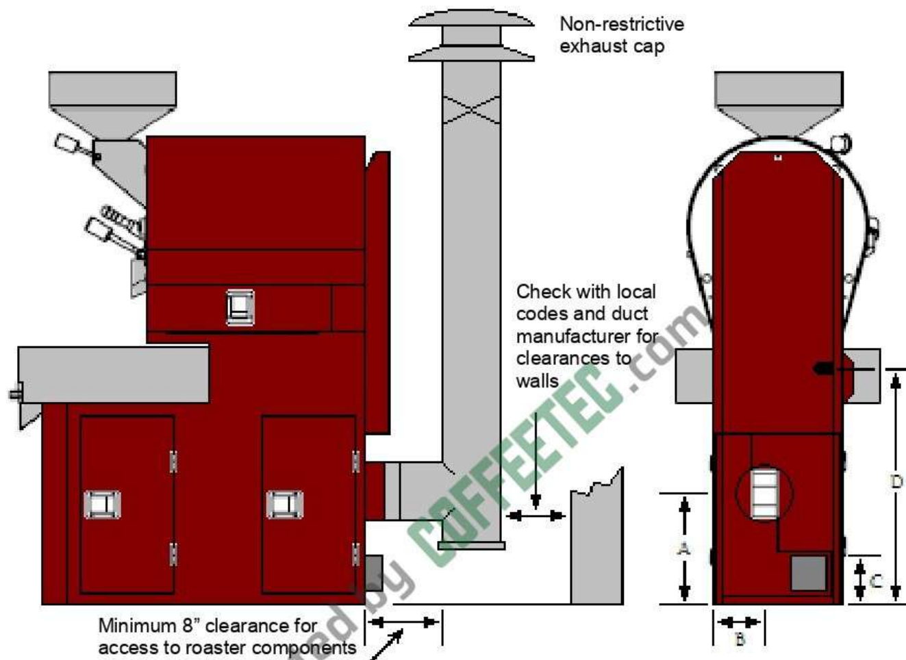
Roaster Models - Dimensions in Inches / Centimeters
