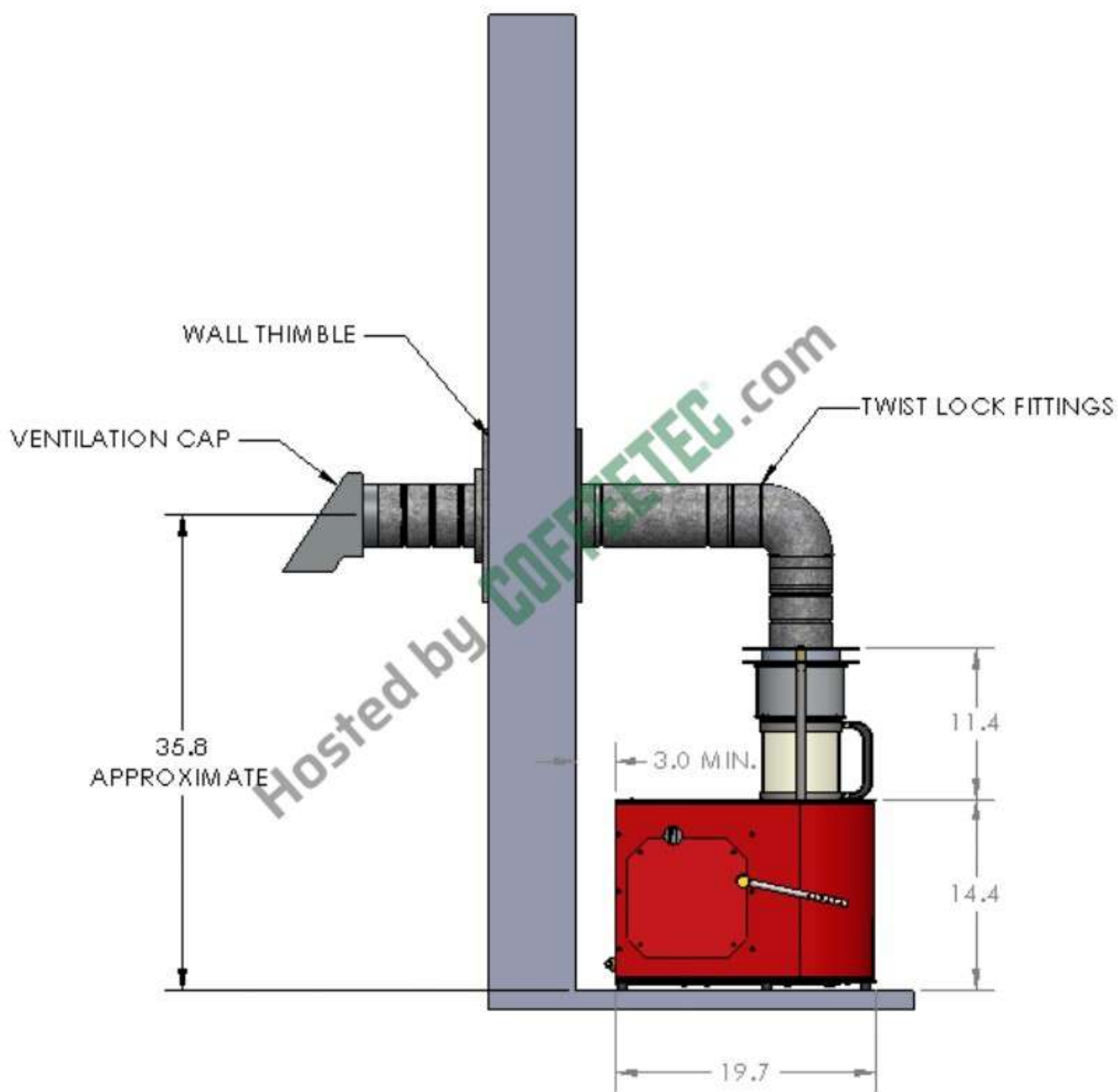
TYPICAL DIRECT VENT INSTALLATION SONOFRESKO VK-100 VENT KIT SHOWN ROASTER WIDTH APPROX. 13.0" WIDE
